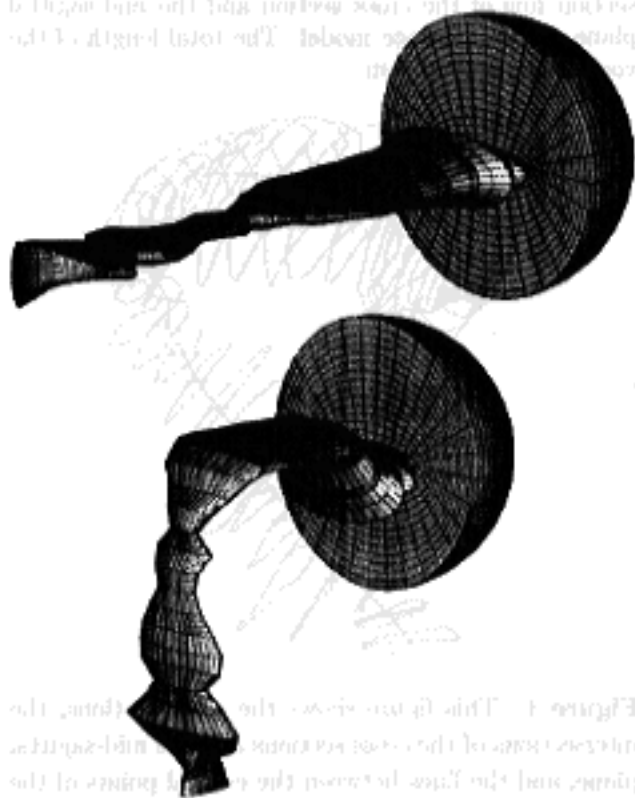
Figure 5: The FE meshes of the elliptical models. top: straight configuration, bottom: bent configuration.
