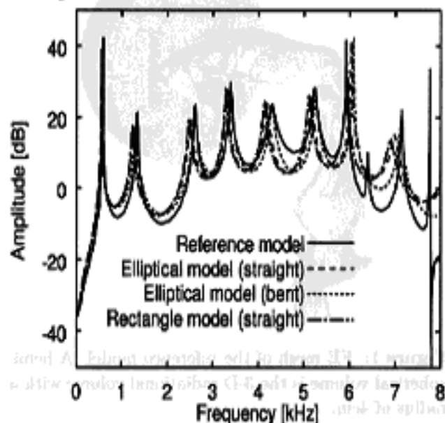
Figure 6: VTTFs from FEM simulation.
