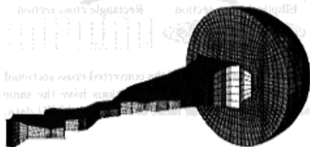
Figure 4: The FE meshes of the rectangle model
